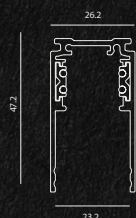
48 V surface mounted deep profile track AC-DN120 Track length 1meter / 2meters
